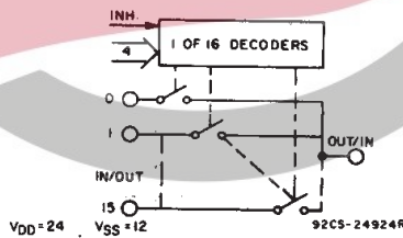
Fig. 1 – CD4067 functional diagram.
